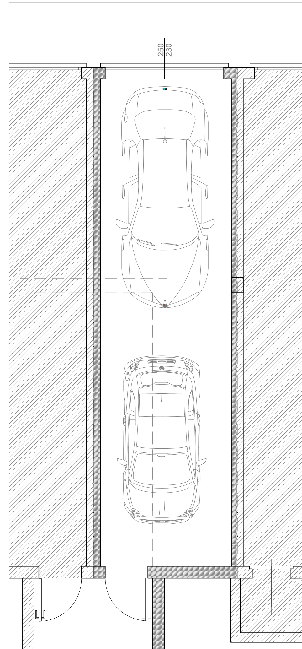
PIANO INTERRATO
