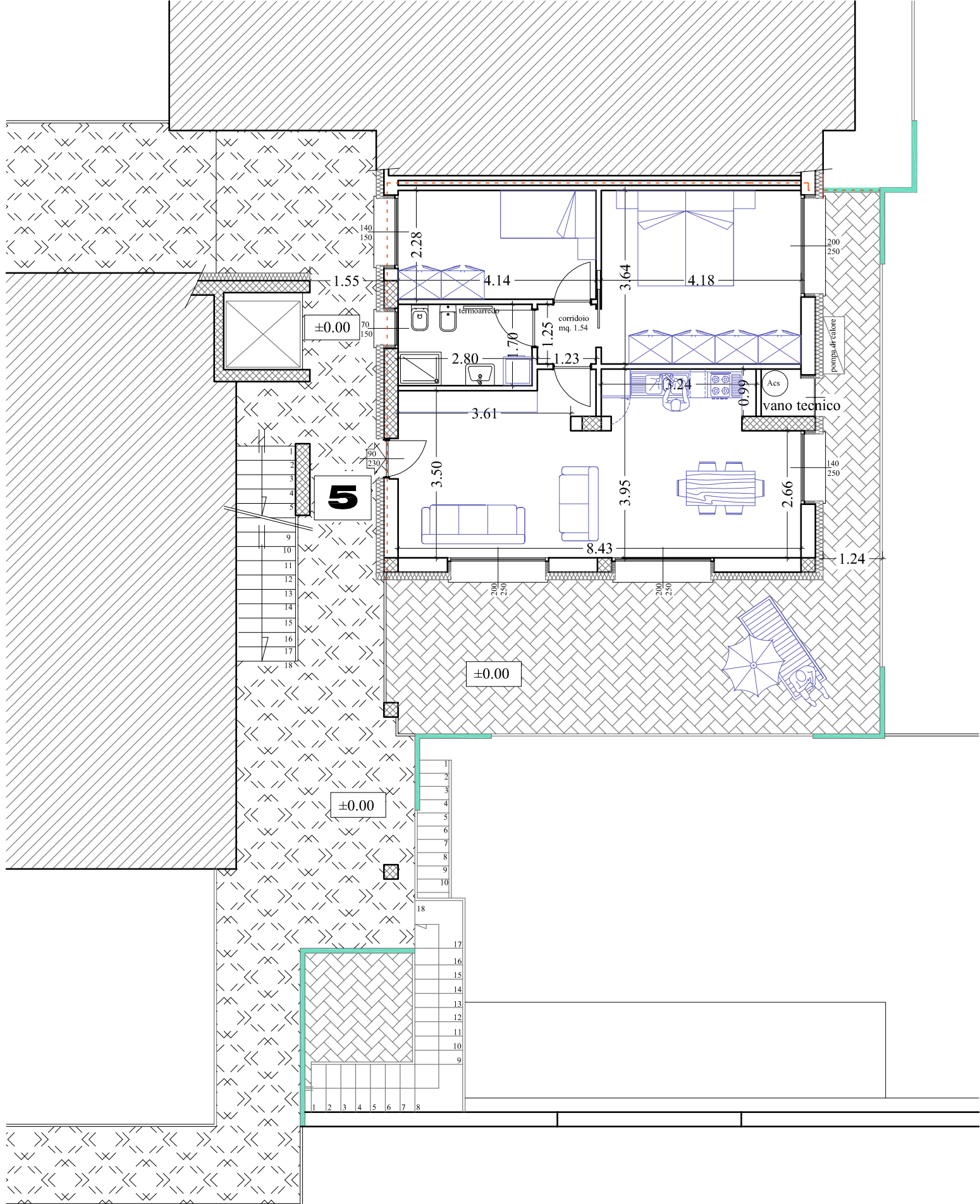
RESIDENCE " CERVINO " - CANTU' APPARTAMENTO - 5 - scala 1 : 100
